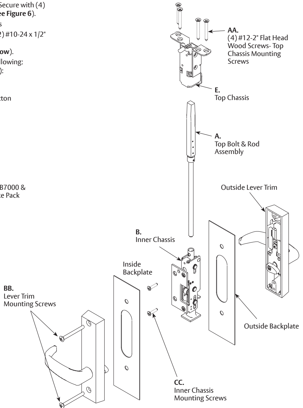
Figure 6: NB-WD7000 Assembly Exploded View
