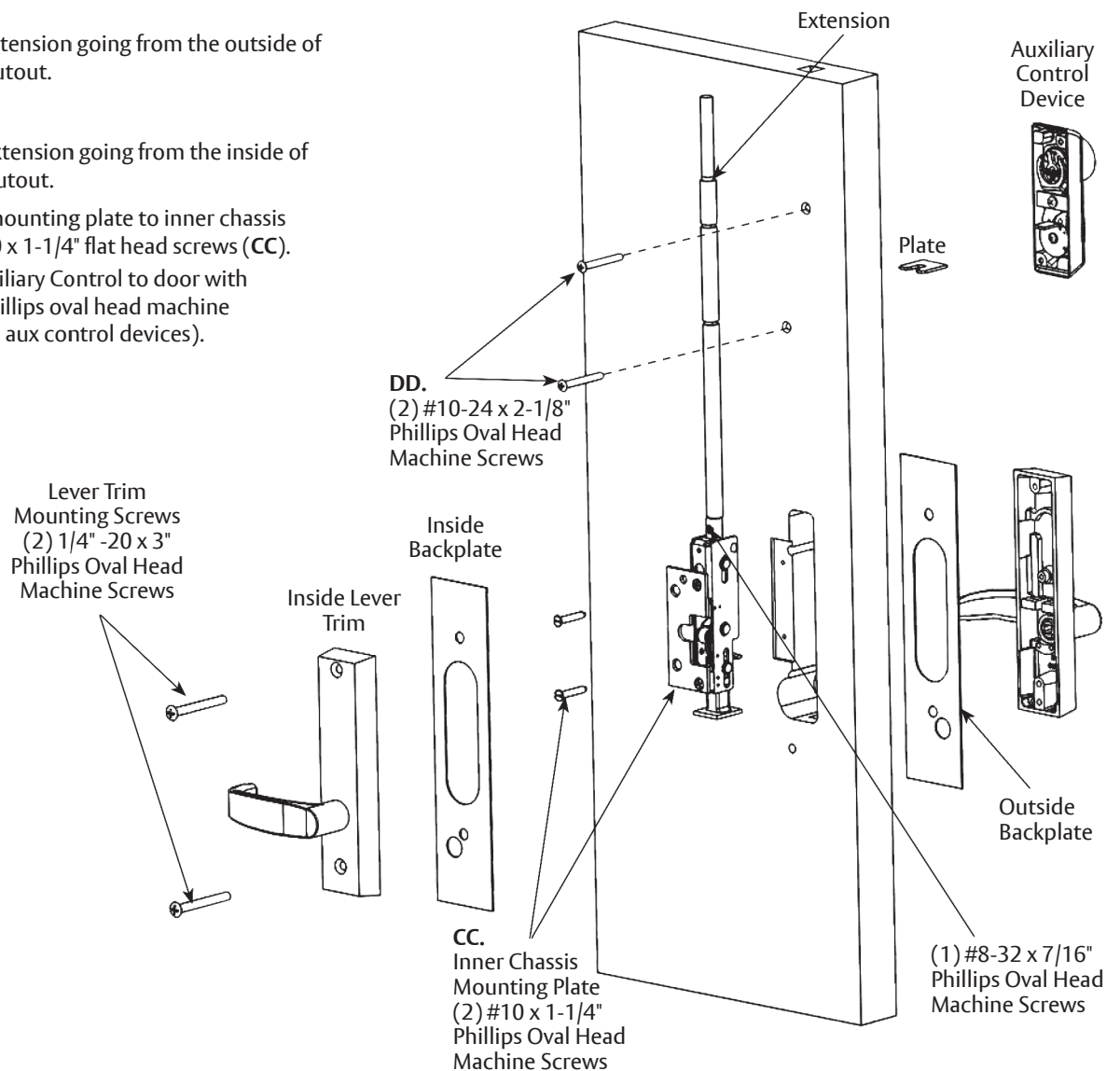
Figure 9: WD7000 Trim Assembly Exploded View
