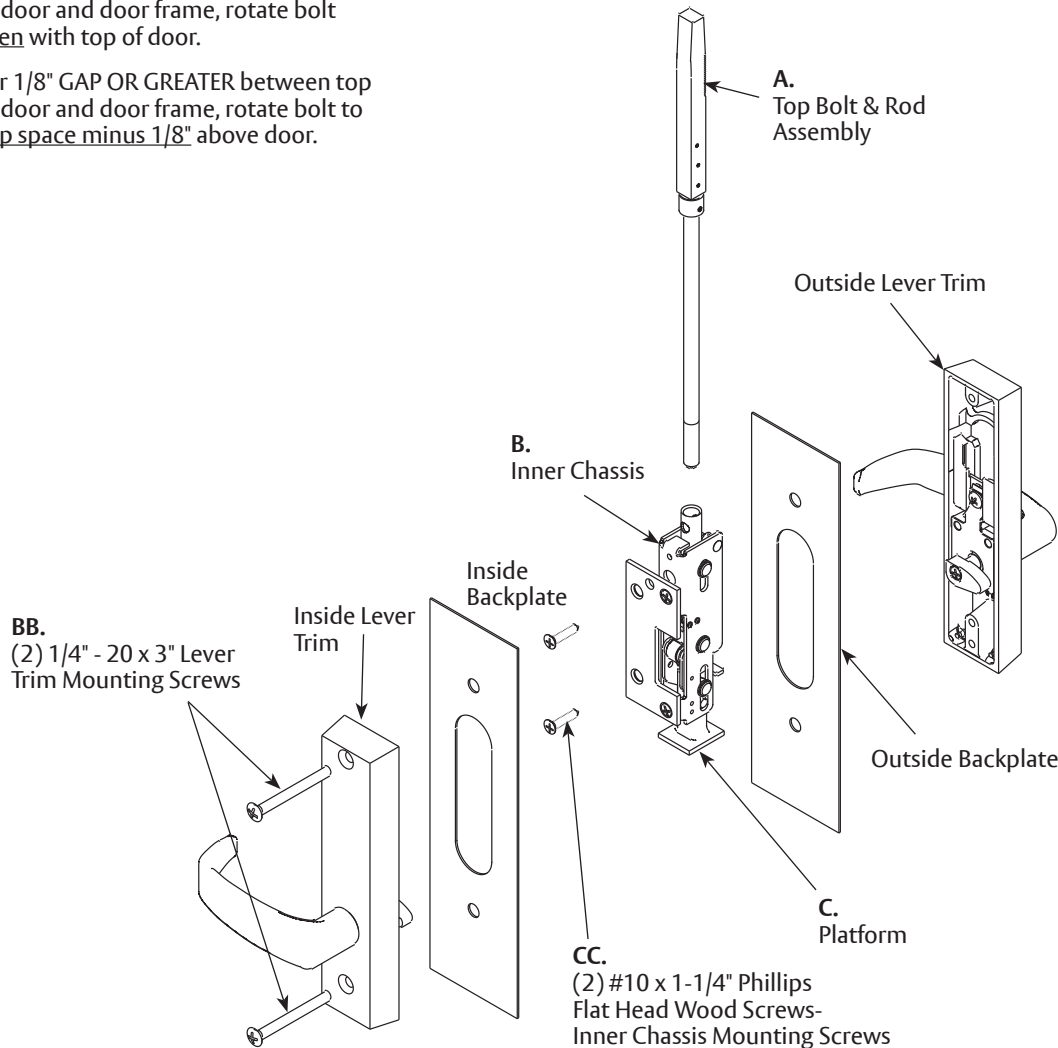
Figure 5: NB-WD7000 Assembly Exploded View
