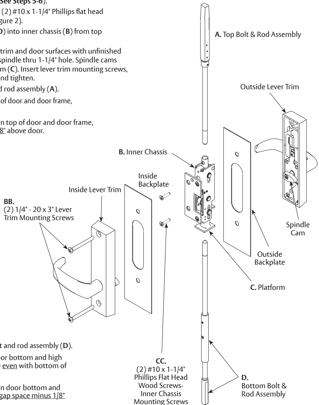
Figure 2: WD-7000 Assembly Exploded View
