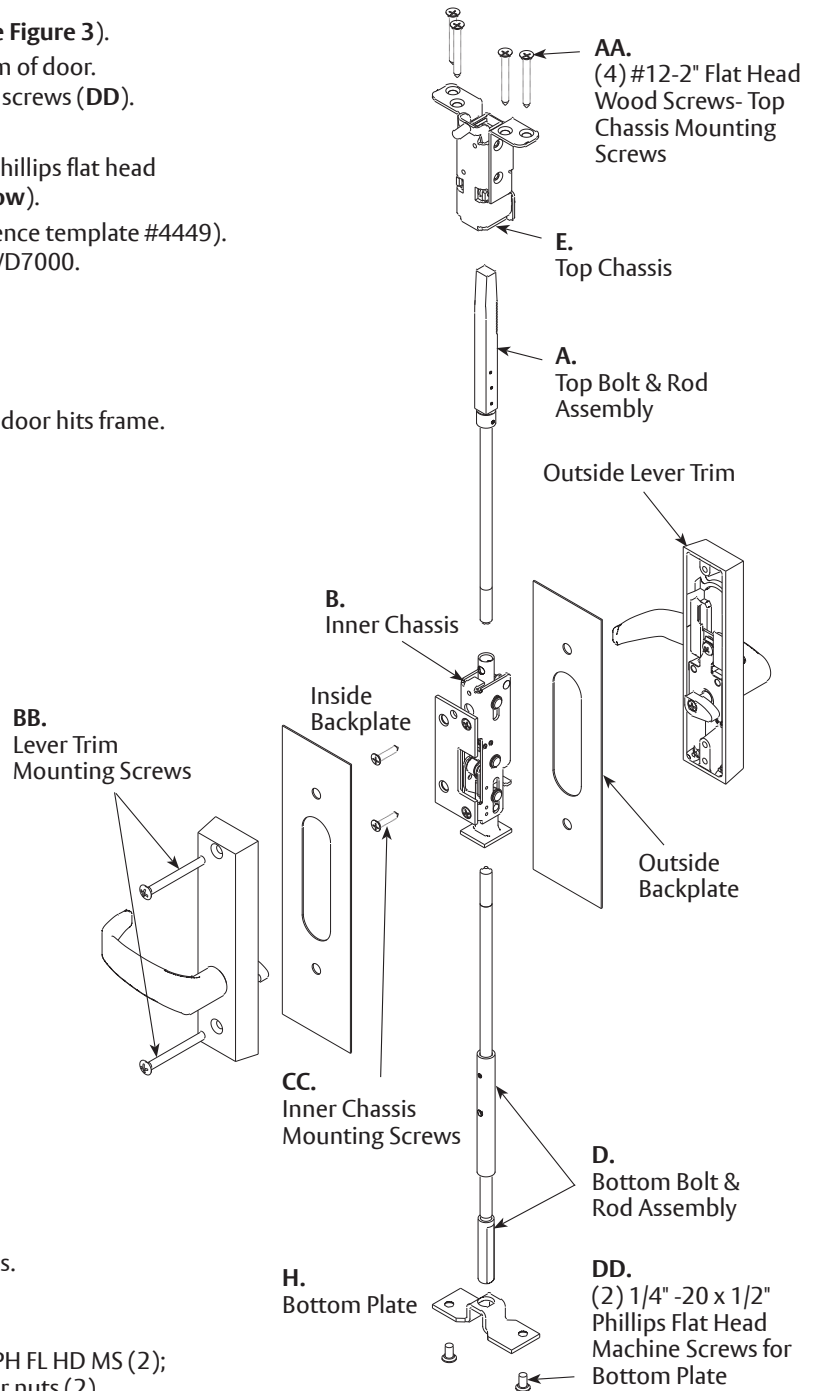
Figure 3: WD-7000 Assembly Exploded View
