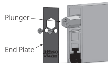
Figure 5 Plunger end plate prevents the plunger adjustment from rotating.
