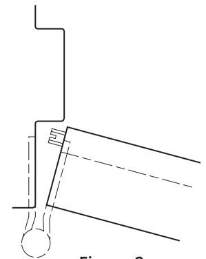
Figure 2 Semi-Mortise Mounted
