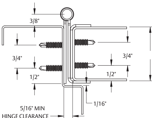
Fig. 2 HINGE PLACEMENT & CLEARANCE TEMPLATE (NON-ADJUSTABLE APPLICATION SHOWN)
